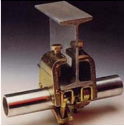
Girder Coupler Fixing
